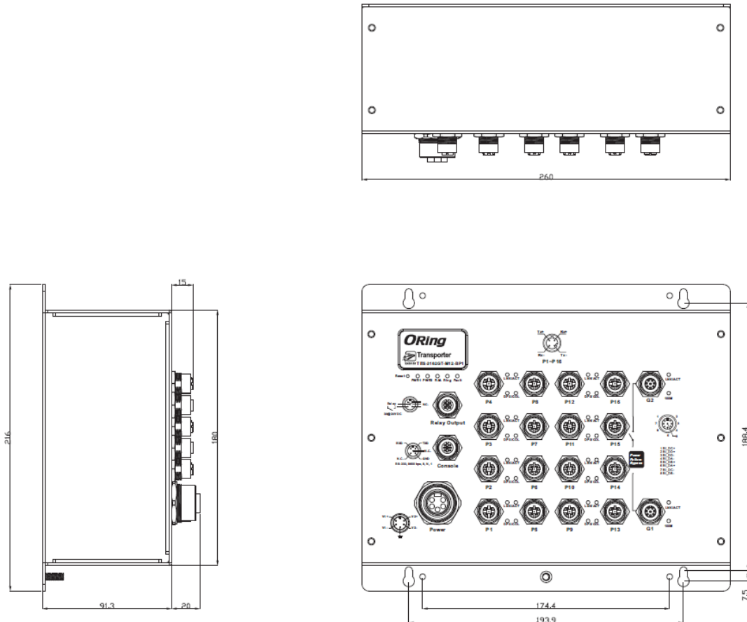
Wall-mount Kit Measurements (Unit = mm)
