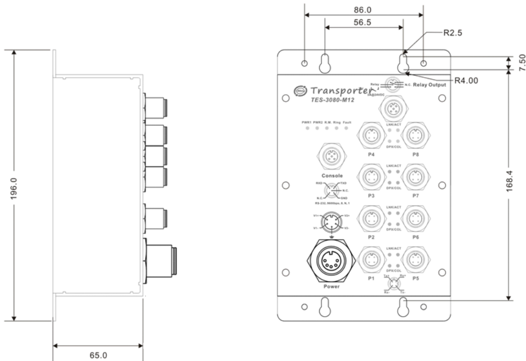
Wall-mount Measurements
